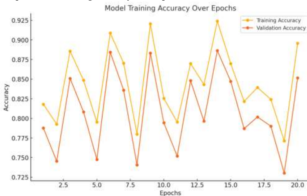
Graph: Model Training Accuracy Over Epochs
